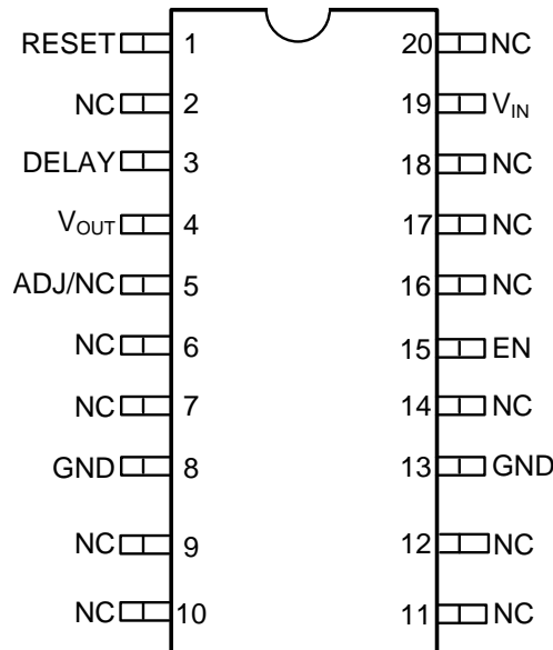
20-Terminal HTSSOP PWP Package (Top View)
