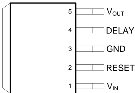
5-Terminal DDPK KTT Package Fixed Version A (Top View)
