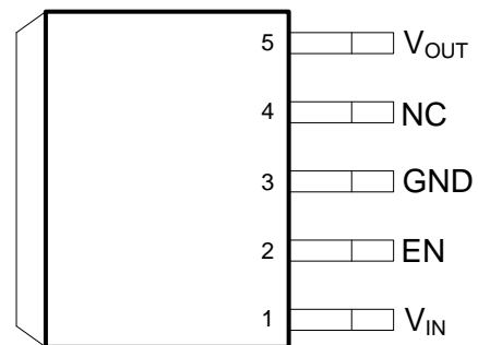
5-Terminal DDPK KTT Package Fixed Version B (Top View)
